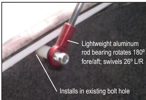
911/912 trunk - uses existing hole; no drilling
